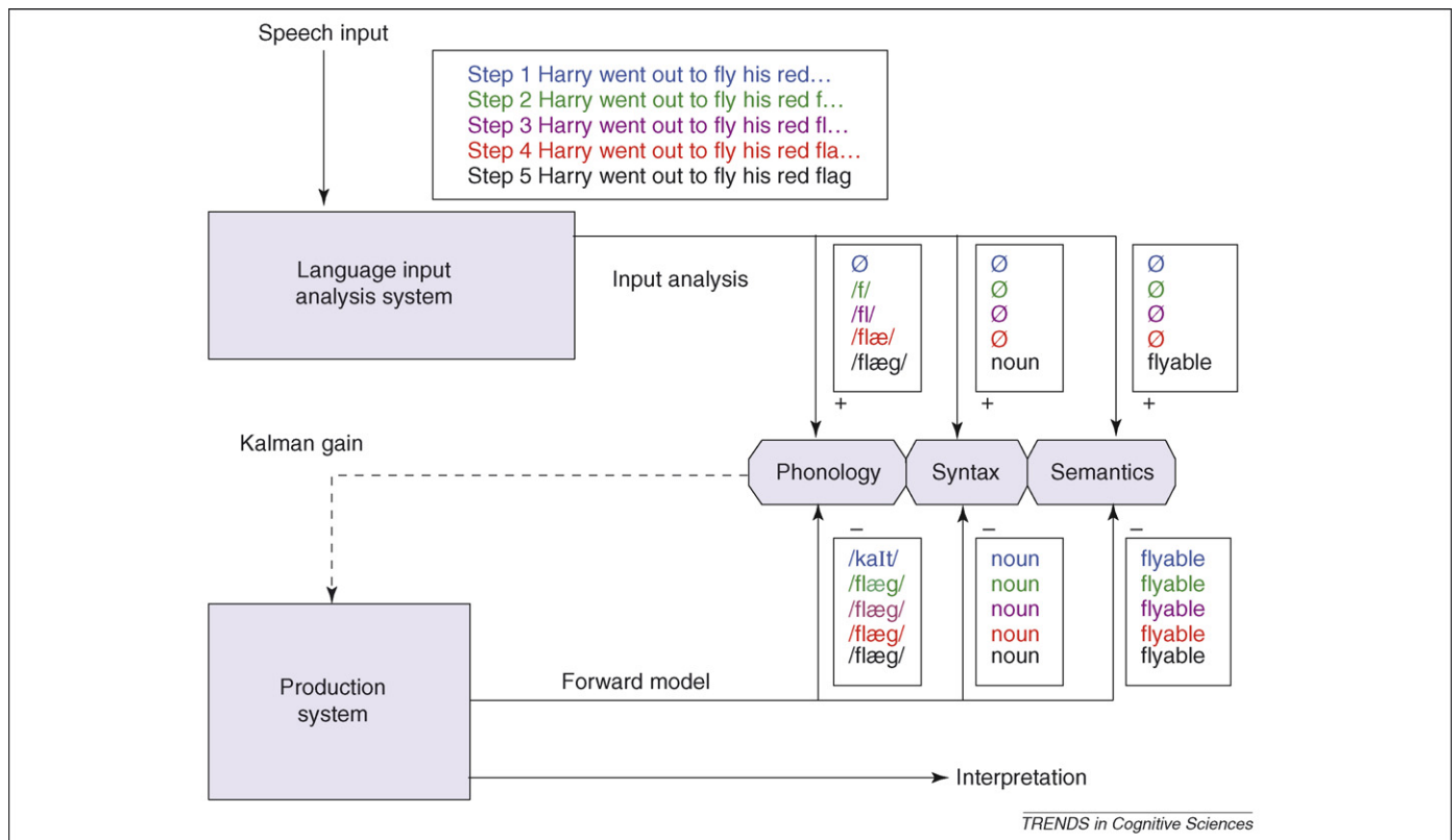
Figure 1. Schematic representation of a production-based language emulator. The emulator is controlled by feedback from a Kalman filter, which weights predictions against analysis of the input at each step. If the prediction is strong and the input noisy, there is low Kalman gain (strong top-down influence on interpretation); if the prediction is poor and the input clear, there is high Kalman gain (strong bottom-up influence). Illustrated are the five steps in comprehending the end of the sentence 'Harry went out to fly his red flag.' At each step, the input analysis and the forward prediction are shown in the same colour for three different levels of prediction (phonology, syntax and semantics). In this case, we make three simplifications. First, the input is noise-free, so that (for instance), at Step 2, the input analysis system is certain that it has encountered /f/ rather than /p/ or /k/. In a noisy environment, it might ascribe a probability of 0.9 to /f/ and 0.1 to other possibilities. Second, we illustrate only a single prediction at each linguistic level, although we assume that a range of predictions are made. In reality, at Step 1, the emulator might ascribe a probability of 0.8 to /kaɪt/ (kite), 0.075 to /flæg/ (flag), 0.1 to /pleɪn/ (plane) and 0.001 to each of various other possibilities; at Step 2, the probability of /flæg/ might go up to 0.95, and so on. By contrast, the probability of the sentence ending in a noun is (virtually) 1 at Steps 1–5. Third, we ignore the possible complexity of the semantic representations (e.g. how fine-grained they are).
